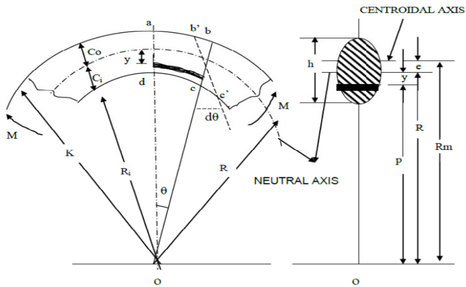
FIG.1 CURVED BEAM SUBJECTED TO BENDING MOMENT
