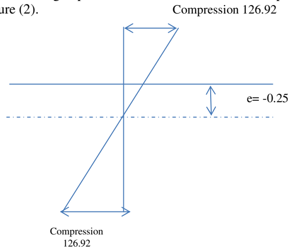
Figure (2): Eccentricity for Trapezoidal section is minimum
