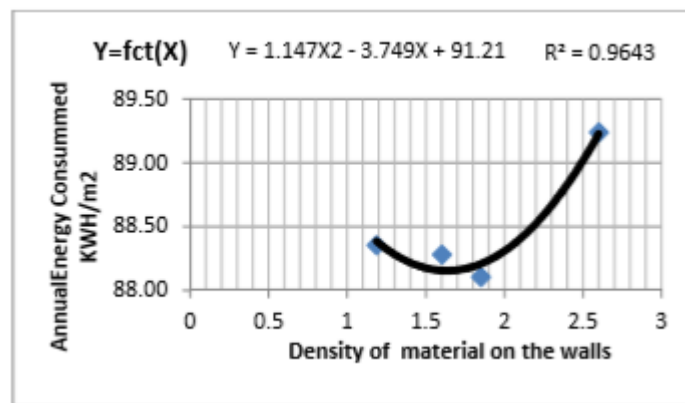
Figure 12 Curve correlation between energy consumed in the building and the density of wall's material in tropical Sudano Sahelian climate
