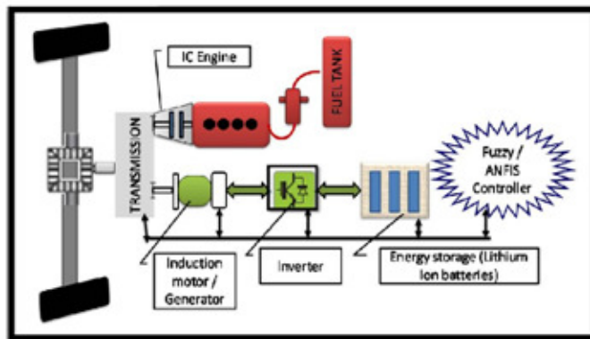
Figure 1 The schematic of proposed hybrid system
