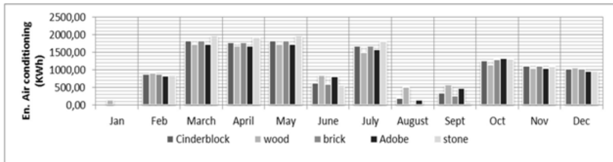
Figure 8 annual variations in cooling energy consumption in tropical dry climate The final energy consumption balance sheet is presented in Table 12:
