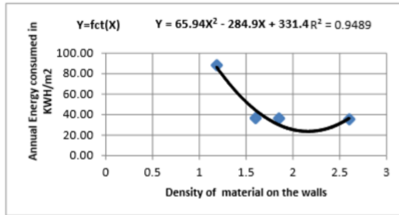
Figure 14 Curve correlation between energy consumed in the building and density of the walls of the material in Equatorial Guinea climate
