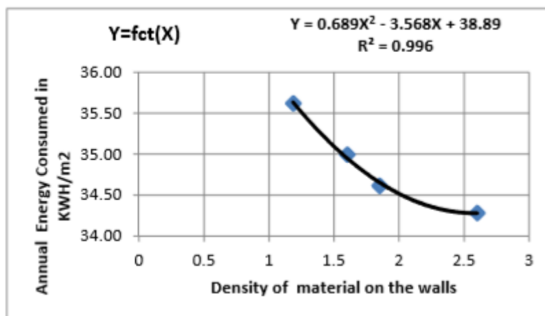
Figure 13 Curve correlation between energy consumed in the building and density of the wall's material in a humid tropical climate
