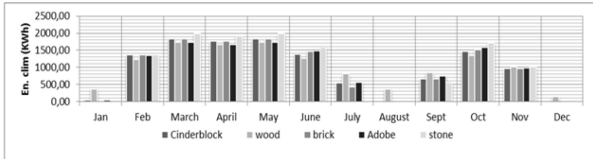
Figure 9 annual changes in cooling energy consumption in Sudano Sahelian tropical climate The final energy consumption balance sheet is presented in Table 13:
