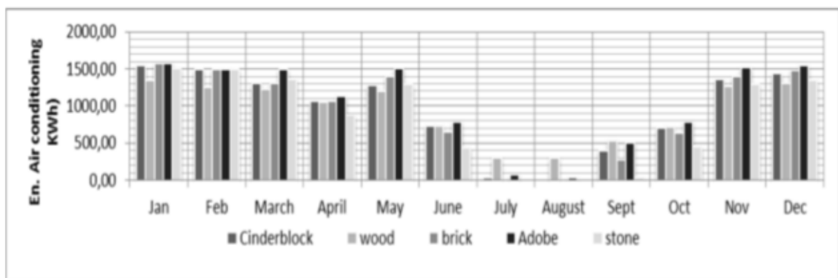
Figure 6 annual changes in cooling energy consumption in the building in Equatorial Guinean climate.
