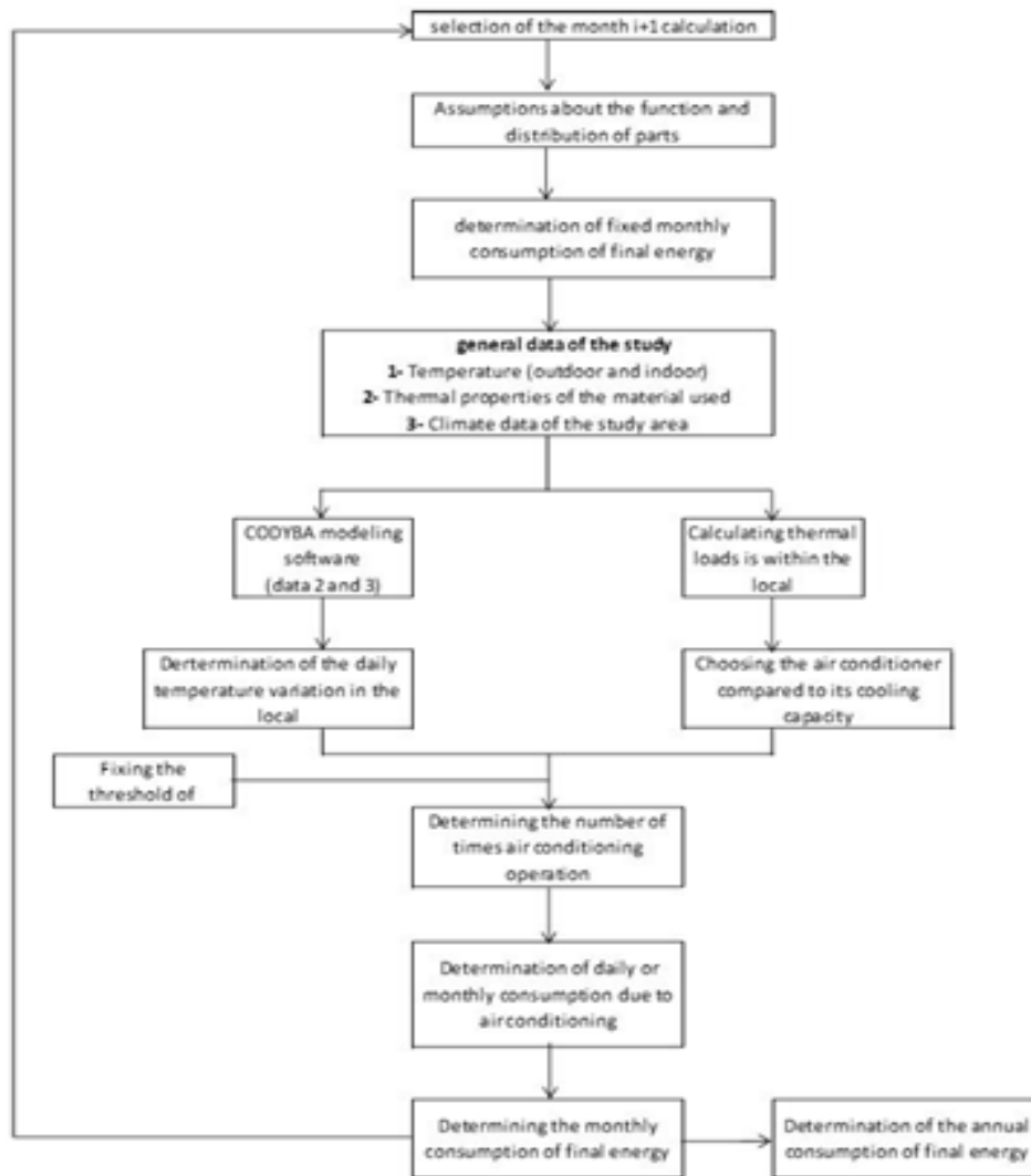
Figure 2 Flowchart for determining the annual energy consumption
