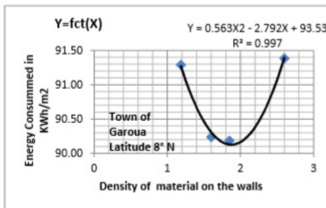
Figure 11 Correlation Curve for the tropical Sudanese climate
