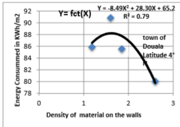
Figure 10 Curve correlation between energy consumed in the building and density of the walls' material in coastal Cameroonian equatorial climate
