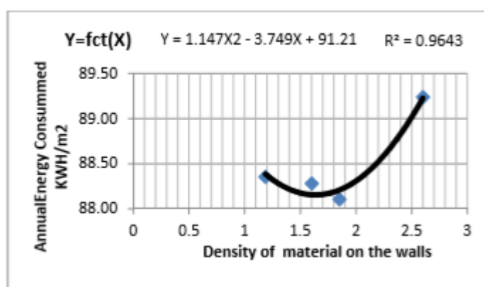
Figure 12 Curve correlation between energy consumed in the building and the density of wall's material in tropical Sudano Sahelian climate
