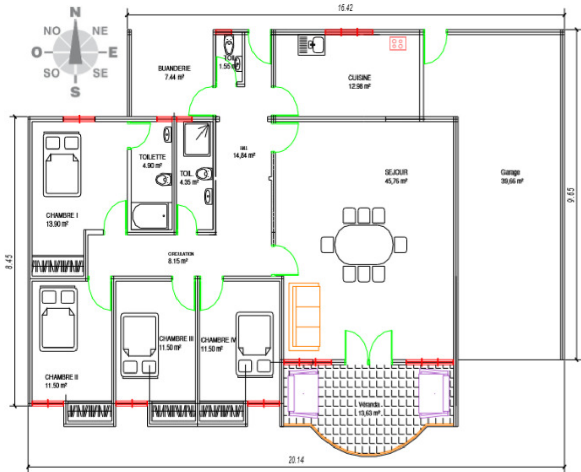
Figure 1 Distribution plan of the pilot building
