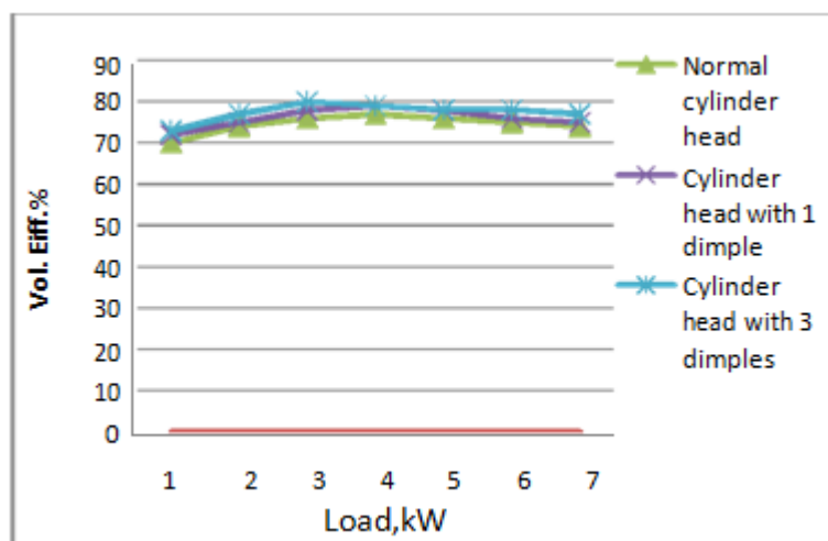
Figure 4 Volumetric efficiency Vs Load
